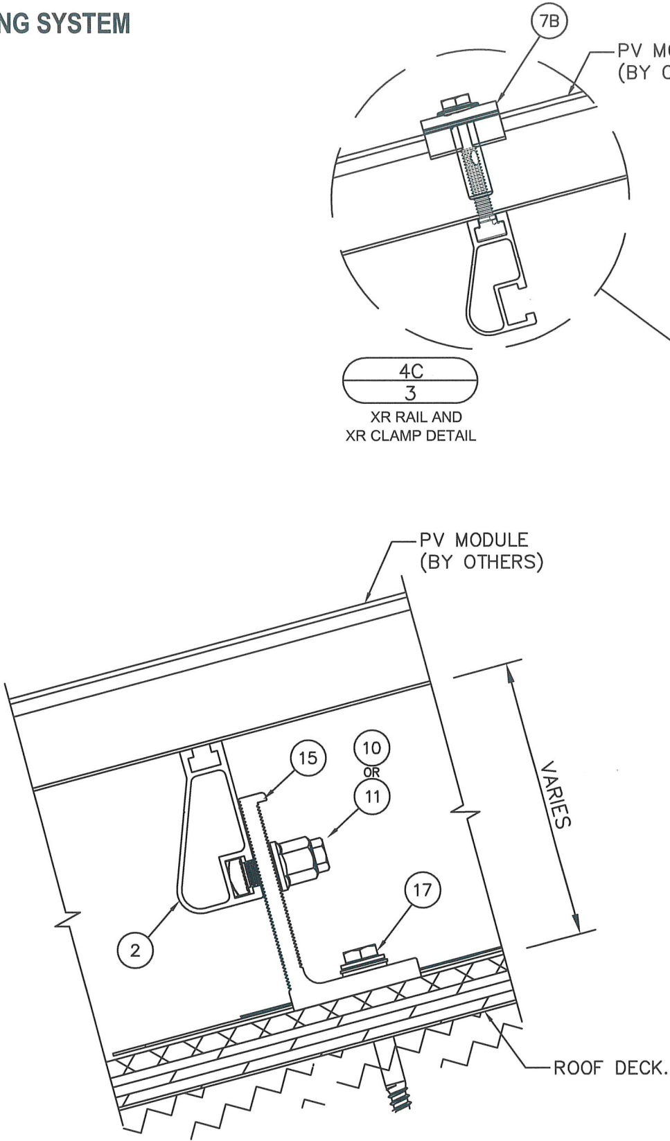
4A 3 XR RAIL AND L-MOUNT DETAIL
