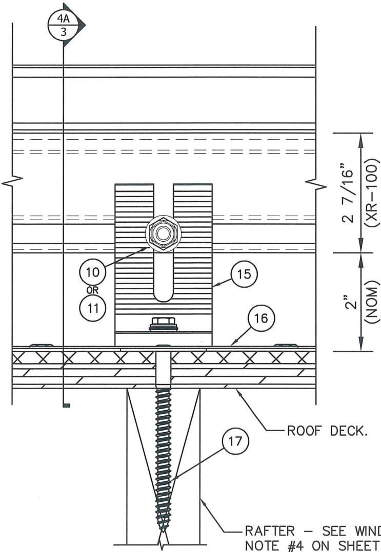
3 3 FLASHVUE DETAIL
